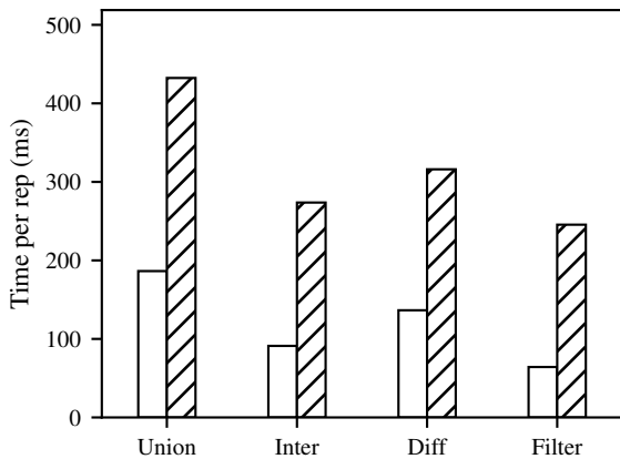
Overhead: stdlib seq vs par (1 domain) (IC1, n = 1M )
