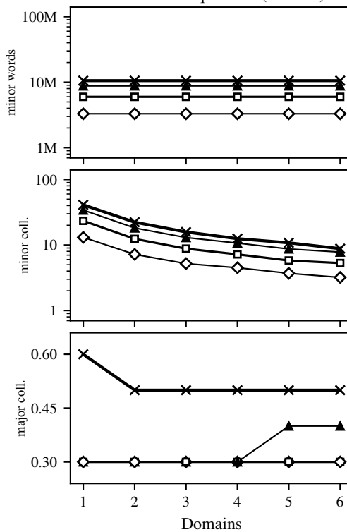
IC4: sorted disjoint ( n = 1M )
