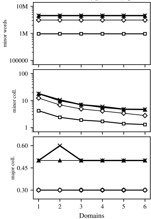
IC3: skewed ratio 9:1 ( n_a = 900k , n_b = 100k )
