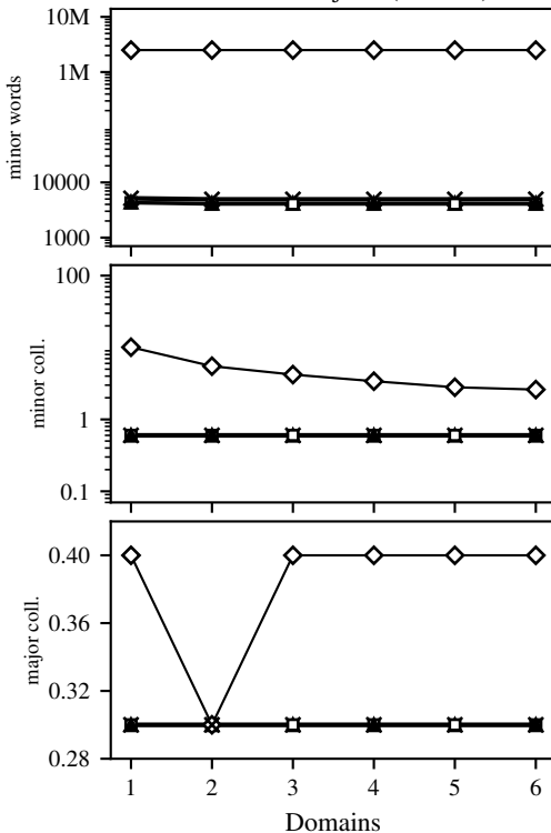
IC4: sorted disjoint ( n = 1M )
