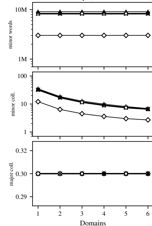
IC5: clustered keys ( n = 1M, 20 clusters)
