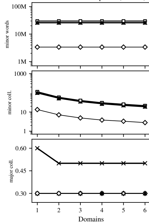
IC2: controlled overlap 50% ( n = 1M )
