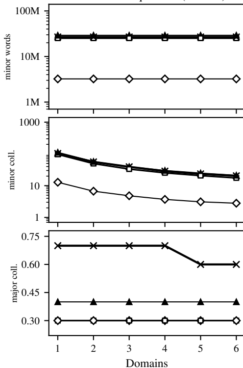
IC1: random equal-size ( n = 1M )
