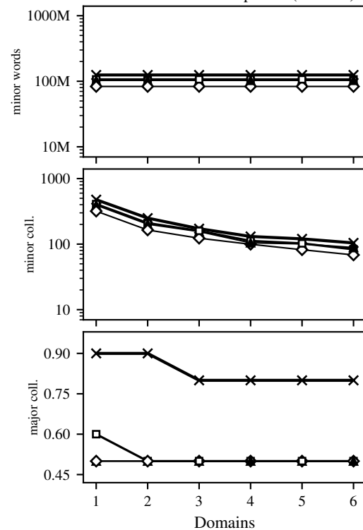
IC2: controlled overlap 50% ( n = 1M )
