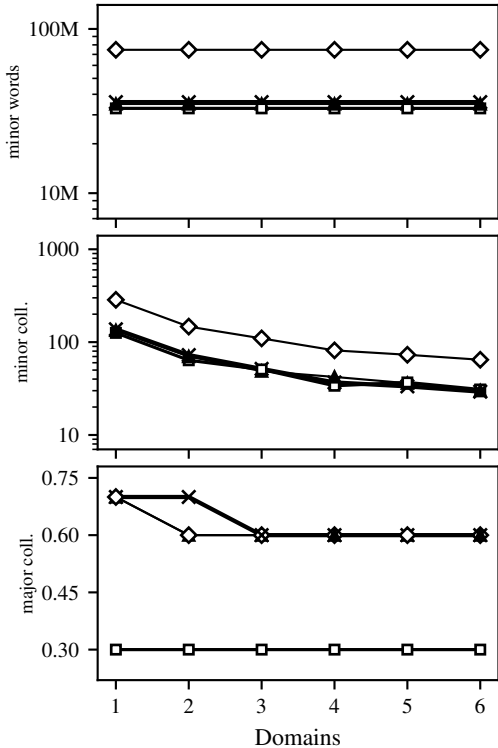
IC3: skewed ratio 9:1 ( n_a = 900k, n_b = 100k )
