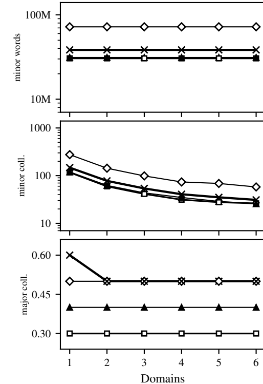
IC5: clustered keys ( n = 1M, 20 clusters)
